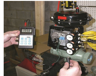
CONTROL VALVES
