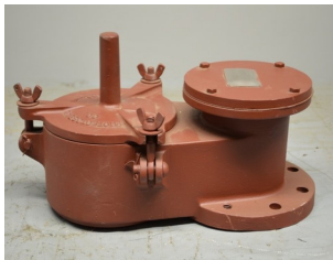
TANK VENTS
