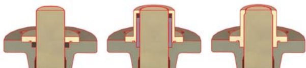
Model 28KV Radial soft seal in the valve body
