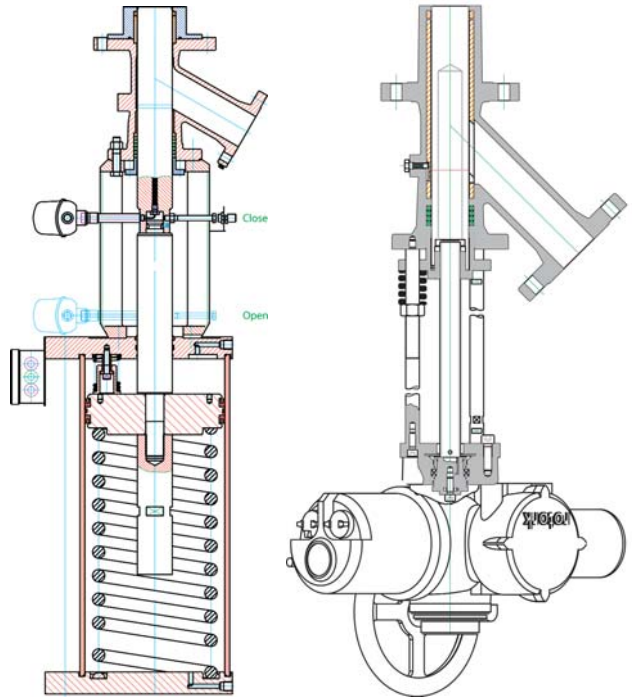
Ram drain valve – Model 28KR
