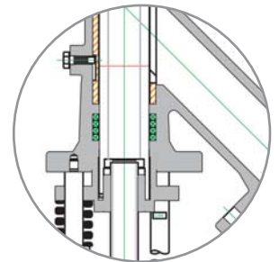
Detail: 26FR – Super Closure
